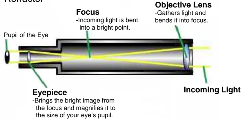
Refractor
